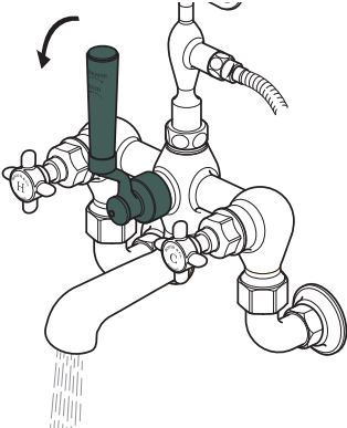
Turning the handle anti-clockwise diverts the water to the spout.
